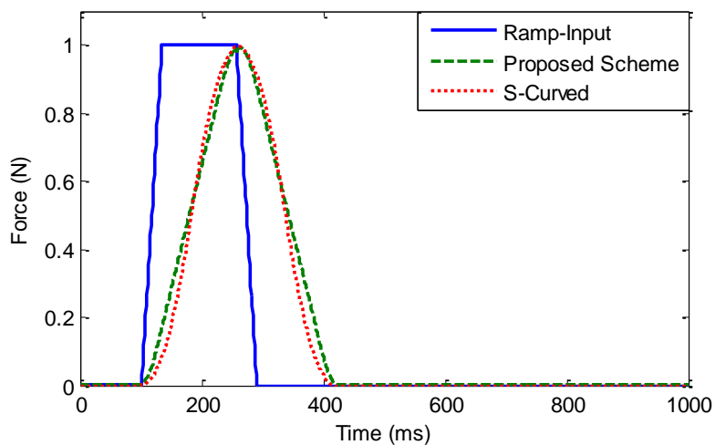
Figure 7. Ramp input, gain-delay shaped and proposed shaped signal (UM-ZV)
