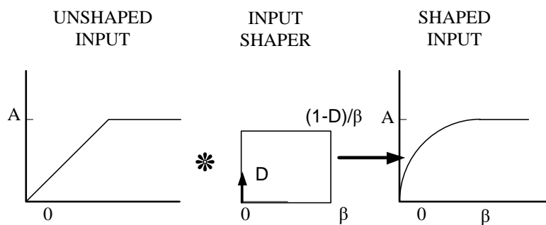
Figure 6. DZV based S-Shaped producing procedure
